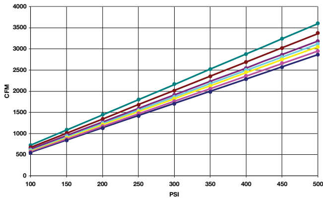
Dominator 1000 Air Consumption
